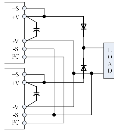
(d) N+1 redundant connection with programmed output and adjustable output voltage
