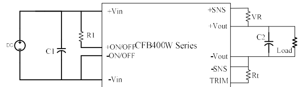
Output Voltage Trim Circuit Configuration
