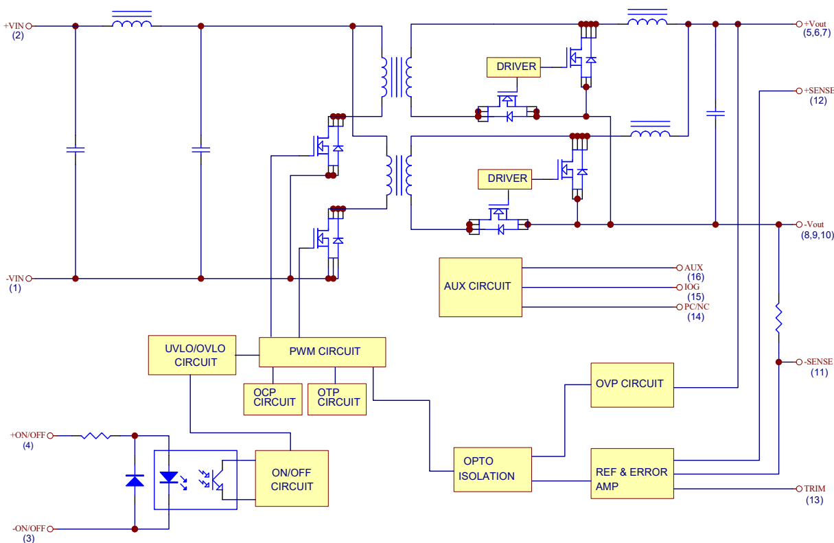
Electrical Block Diagram for 5V Modules
