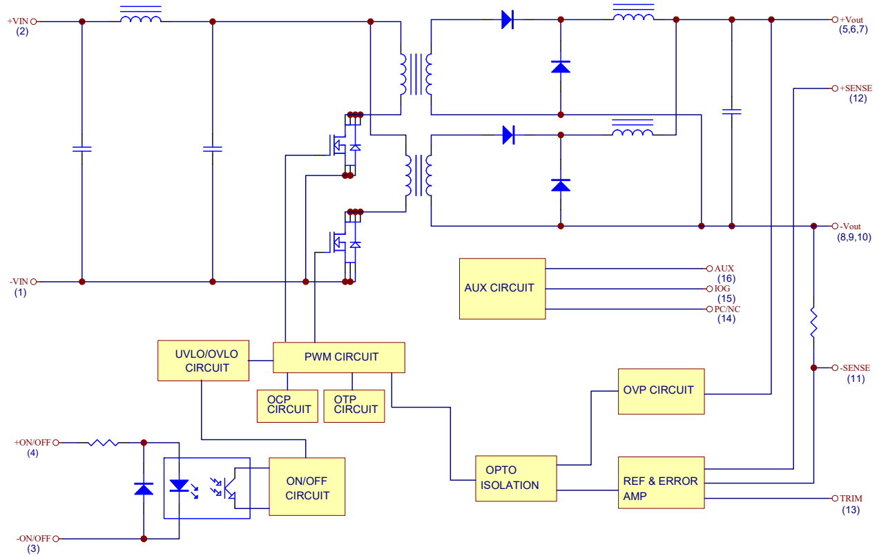
Electrical Block Diagram for other Modules
