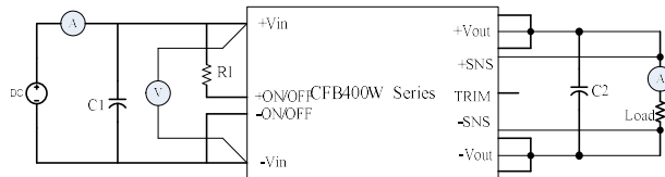
CFB400W Series Test Setup
