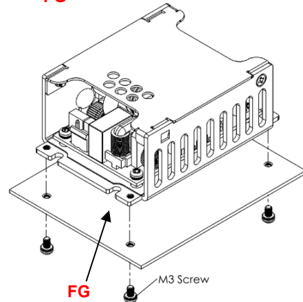
CFM130MXXX-C installation diagram
