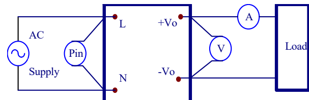
Figure 1. CFM300M Series Test Setup
