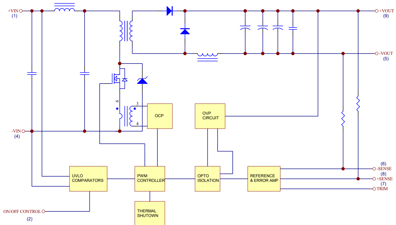
Figure 1 Electrical Block Diagram of CHB150 Series Module
