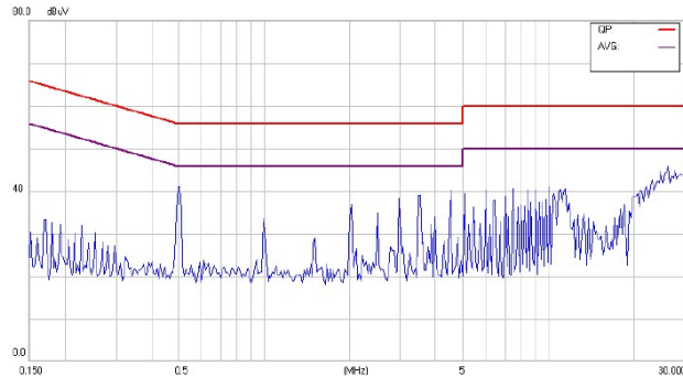
Conducted Class B of CHB150-48S33
