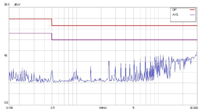
Conducted Class A of CHB150-48S15
