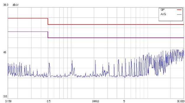
Conducted Class A of CHB150-48S24
