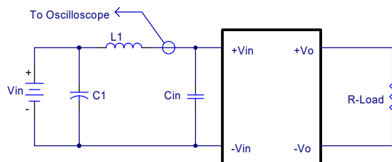
Input Reflected-Ripple Test Setup
