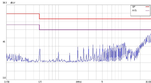
Conducted Class A of CHB150-48S33
