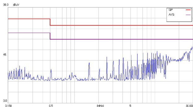
Conducted Class A of CHB150-48S12
