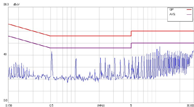
Conducted Class B of CHB150-48S24
