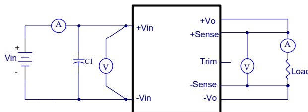
CHB150W Series Test Setup
