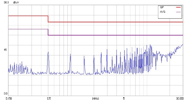
Conducted Class A of CHB150-48S05
