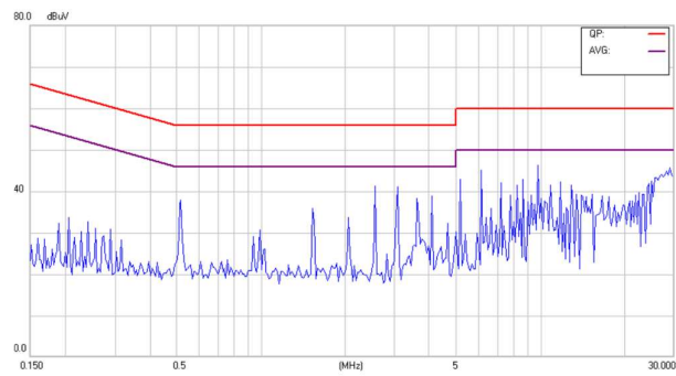
Conducted Class B of CHB150-48S12
