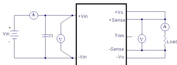
CHB50W Series Test Setup
