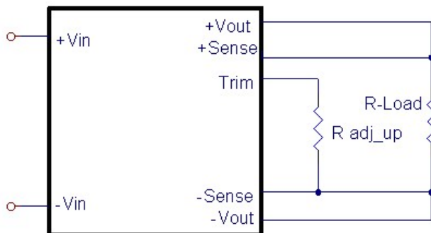
Trim-up Voltage Setup
