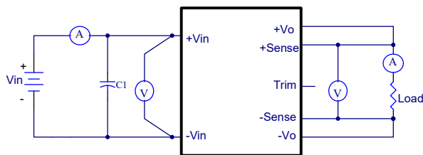
CHB75 Series Test Setup
