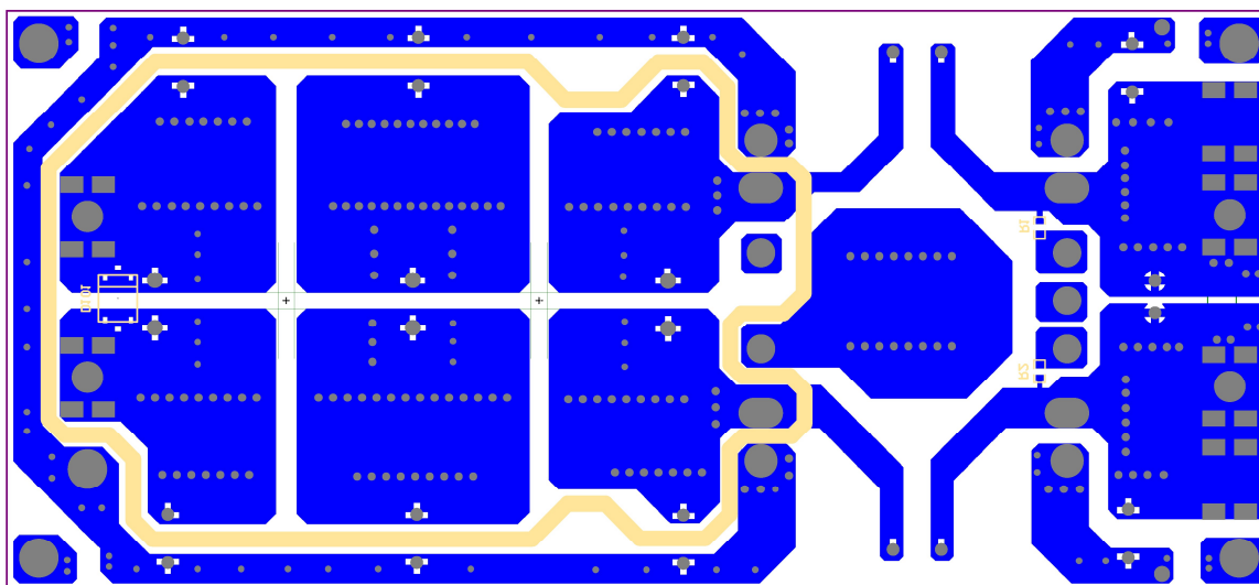
EMI Test Board PCB Layout Bottom View
