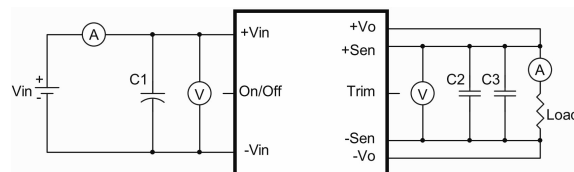
CQB150W Series Test Setup
