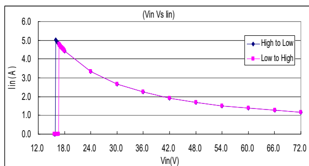
CQB150W-48SXX I in Vs Vin
