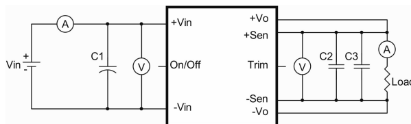
CQB60W-110S Series Test Setup
