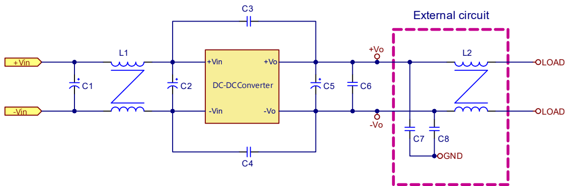
Figure2 Connection Circuit
