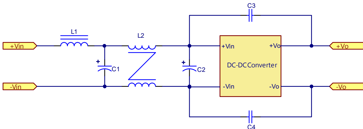
Figure1 Connection Circuit
