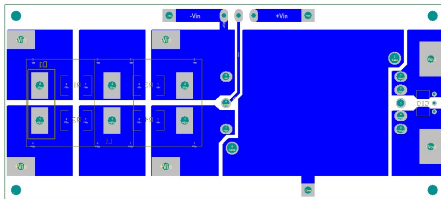
Figure4 PCB Layout Bottom View
