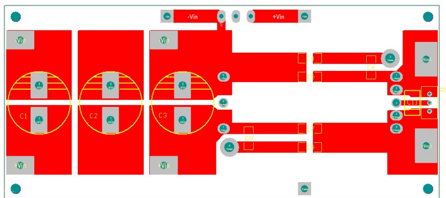
Figure3 PCB Layout Top View
