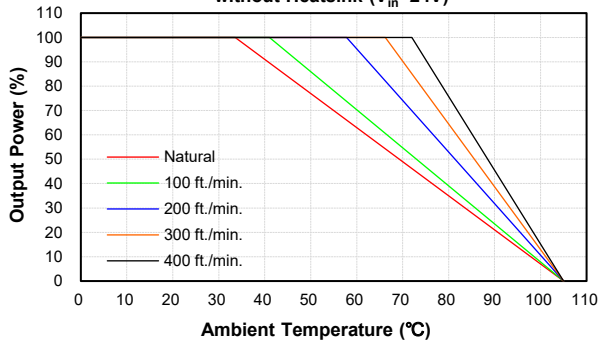
CEB100W-24S12, 48 Derating Curve without Heatsink ( V_{in}=24V )
