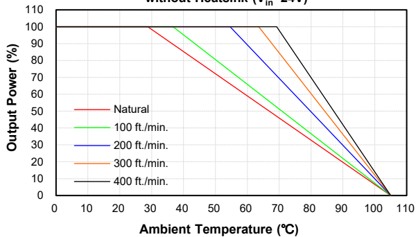
CEB100W-24S24 Derating Curve without Heatsink ( V_{in}=24V )
