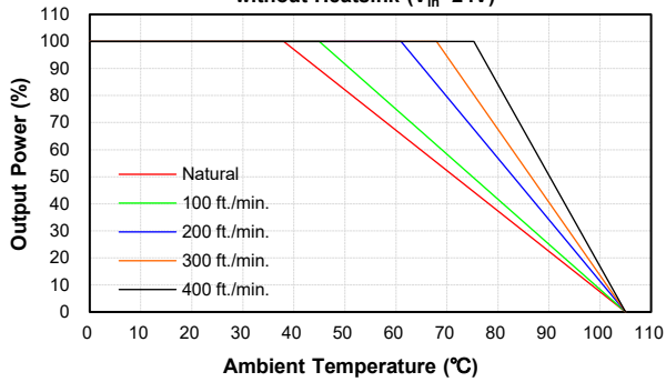
CEB100W-24S05, 54 Derating Curve without Heatsink ( V_{in}=24V )
