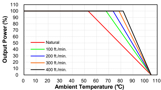
CQB75W14-72S15, 24, 28, 54 Derating Curve with Heatsink QBL127 (Vin=72V)
