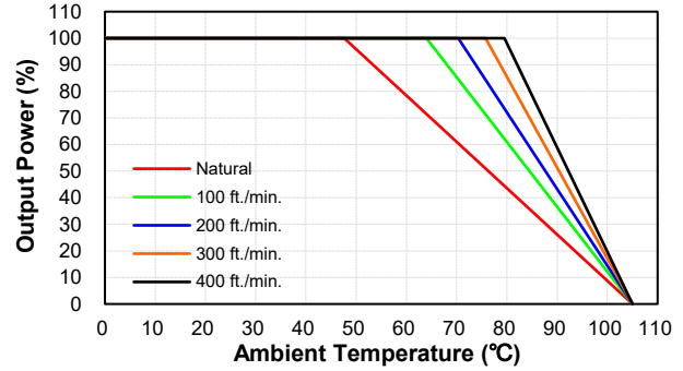
CQB75W14-72S05, 12 Derating Curve with Heatsink QBL127 (Vin=72V)
