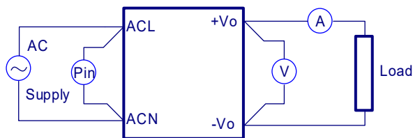
Figure 1. LFM200S Series Test Setup
