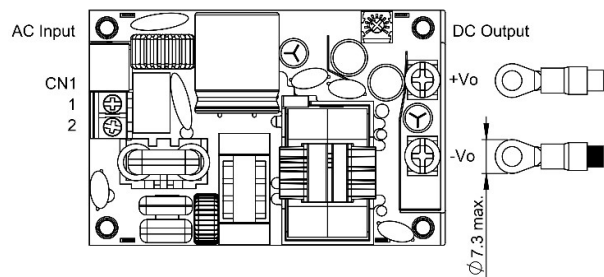
LFM200SXXXB installation diagram
