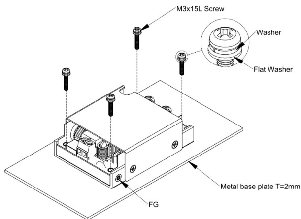
LFM200SXXXC installation diagram
