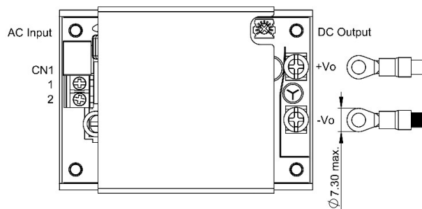
LFM200SXXXC installation diagram
