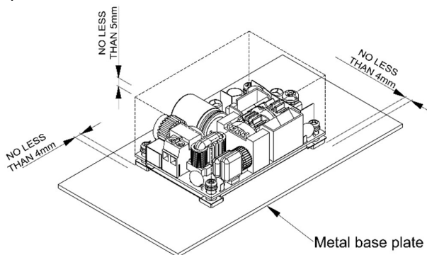
LFM200SXXXB installation diagram
