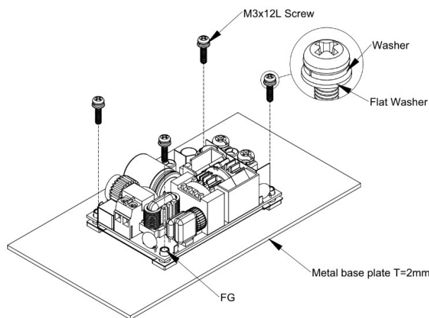
LFM200SXXXB installation diagram
