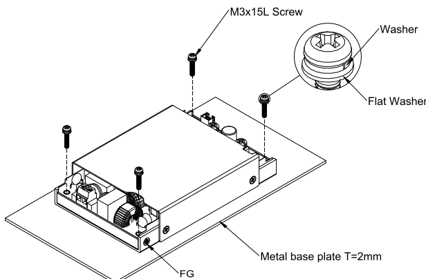
LFM420MXXXC Installation Diagram
