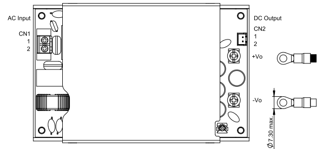
LFM420MXXXC Installation Diagram
