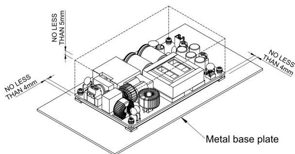
LFM420MXXXB Installation Diagram
