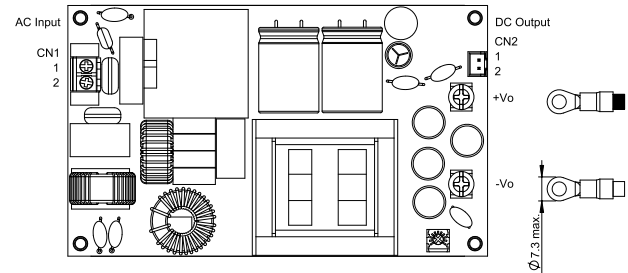
LFM420MXXXB Installation Diagram
