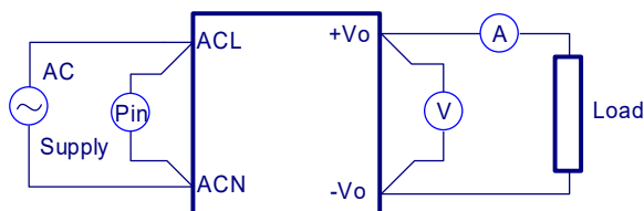
Figure 1. TRE25 Series Test Setup
