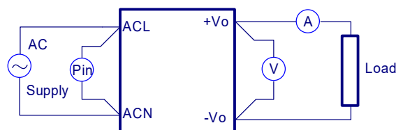
Figure 1. TRE25RD Series Test Setup
