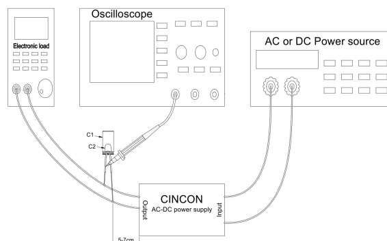
Figure 2. Output Voltage Ripple and Noise Measurement Set up
