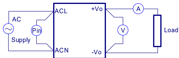
Figure 1. TRH100A Series Test Setup
